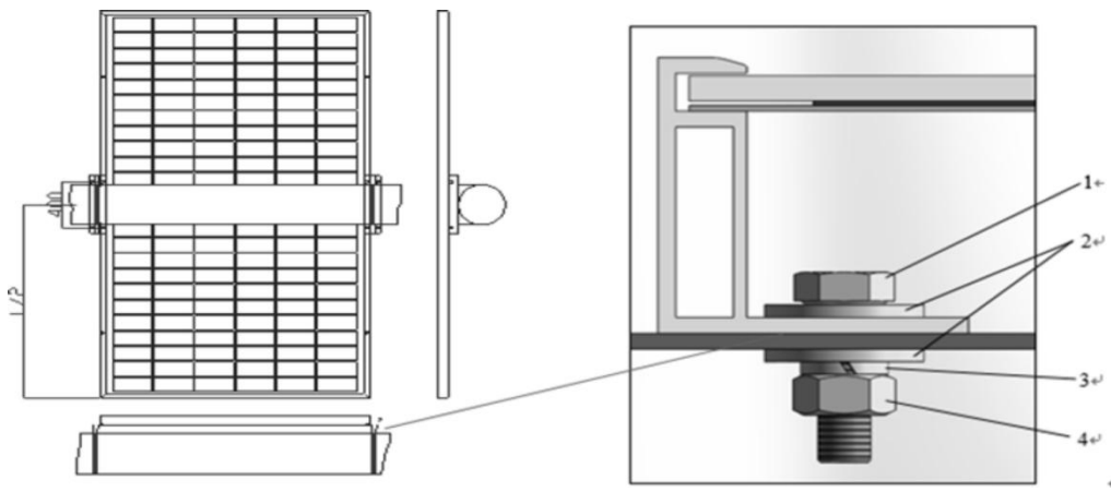
Fig 5-4: PV module installed with Single-axis Tracing System
